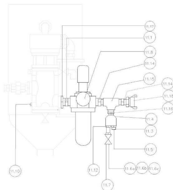
11.0 PRESSURE REGULATOR – PARTS IDENTIFICATION TABLE
