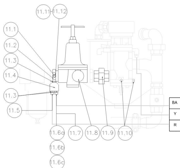
11.0 PRESSURE REGULATOR – PARTS IDENTIFICATION TABLE
